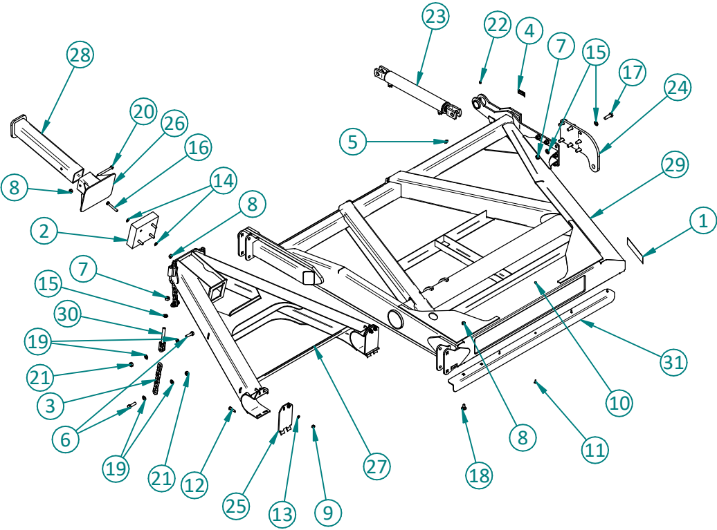
BOTTOM VIEW
