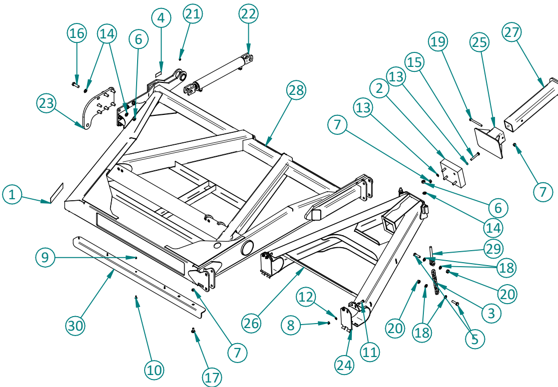
BOTTOM VIEW
