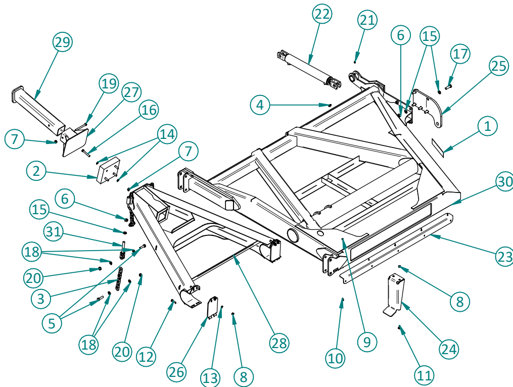
BOTTOM VIEW
