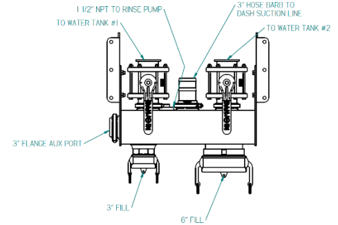
Figure 4.3-Manifold Hose Ports
