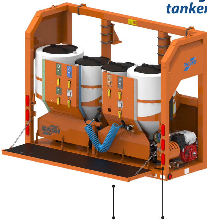
Rear mount includes tail lights and flip down deck.
